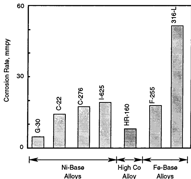
Figure 5. Mass loss data in millimeters per year (mm/yr) for the various alloys exposed to an aggressive chlorinated SCWO feed stream.
