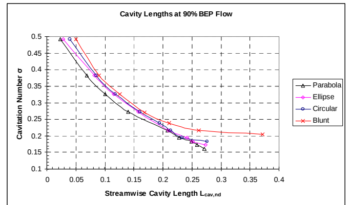
Figure 24: Cavitation bubble growth for different leading edge profiles as NPSH available is reduced; 90% BEP flow at mid-span location
