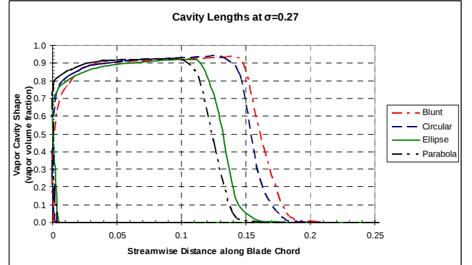
Figure 21: Vapor Cavity Lengths for \sigma=0.27 ; BEP flow at mid-span location.
