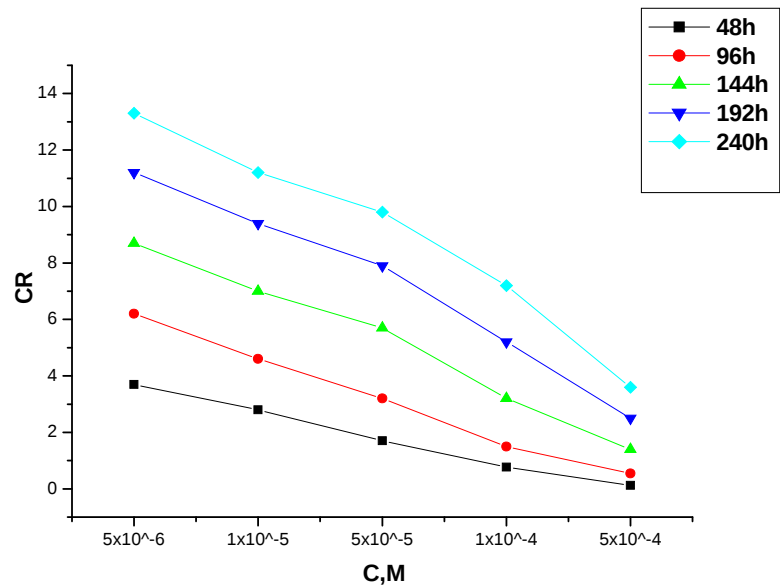
Fig (4): Relation between NHETP inhibitor corrosion rate, inhibitor, concentration.
